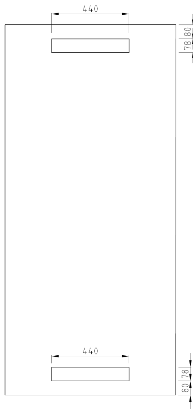
Roosteropening
