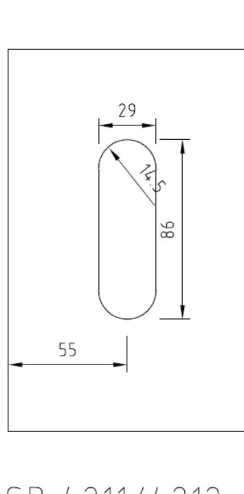
FSB 4211/4212
